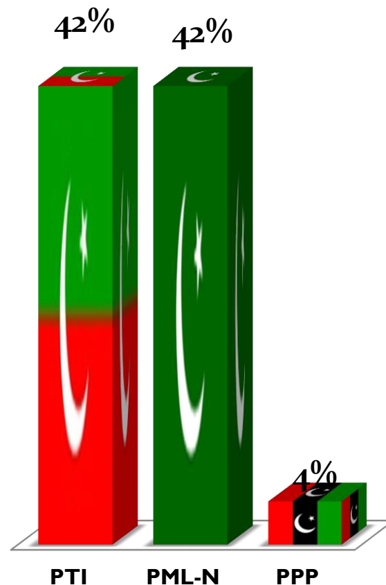
Mean Value (Election 2013+Poll-I)
